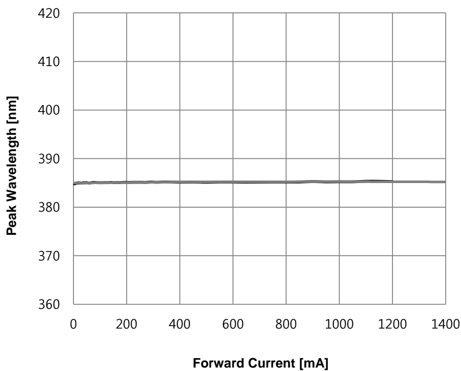
Fig 4. Forward Current vs. Peak Wavelength, T_a=25^{\circ}\text{C}
