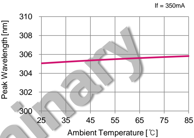
▪ Ambient Temperature vs. Peak Wavelength
